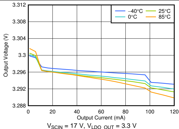
图 5. V_{LDO\_OUT} vs I_{OUT} DC Supply on the SCIN Pin
