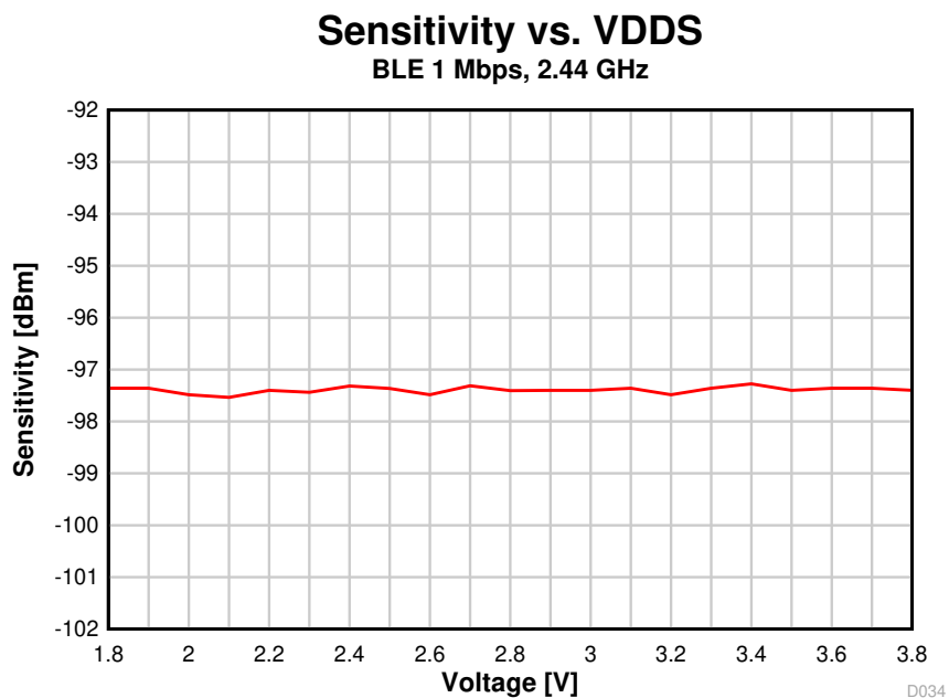
图 8-31. Sensitivity vs. Supply Voltage (VDD5) (BLE 1 Mbps, 2.44 GHz)
