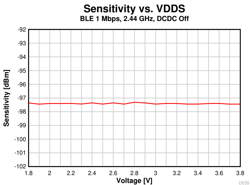
图 8-32. Sensitivity vs. Supply Voltage (VDD5) (BLE 1 Mbps, 2.44 GHz, DCDC Off)
