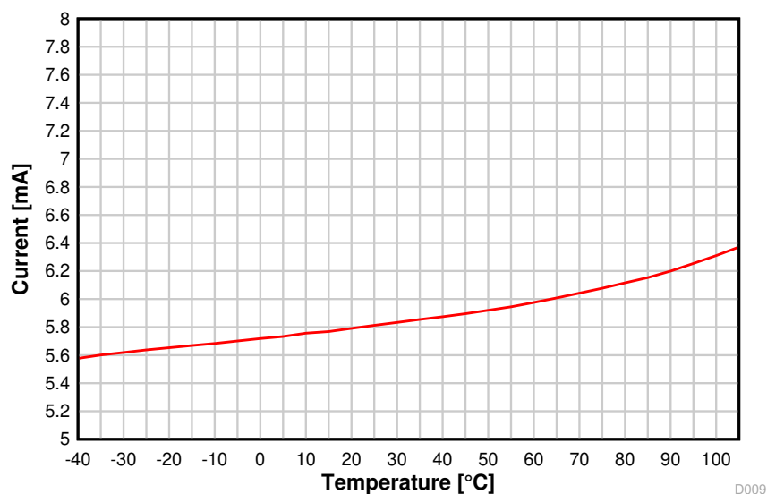
图 8-8. RX Current vs. Temperature (50 kbps, 868.3 MHz, VDD = 3.6 V)
