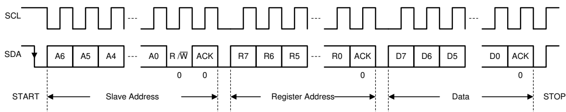
图 6-18. I 2 C Interface WRITE to TPS650861 in F/S Mode
