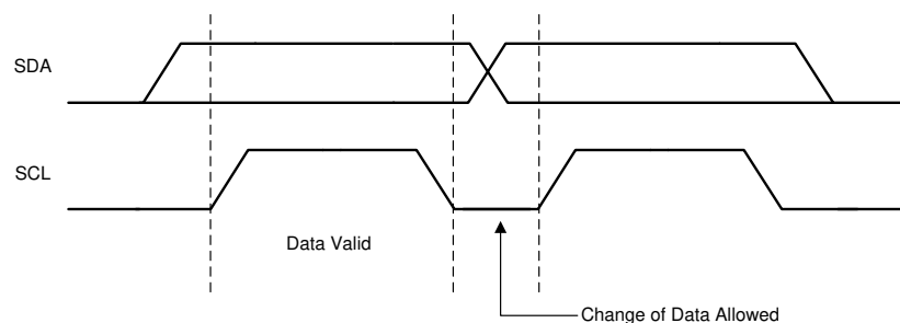
图 6-15. Bit Transfer on the I 2 C Bus
