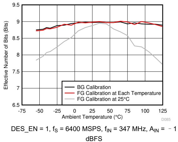
图 6-61. ENOB vs Temperature and Calibration Mode
