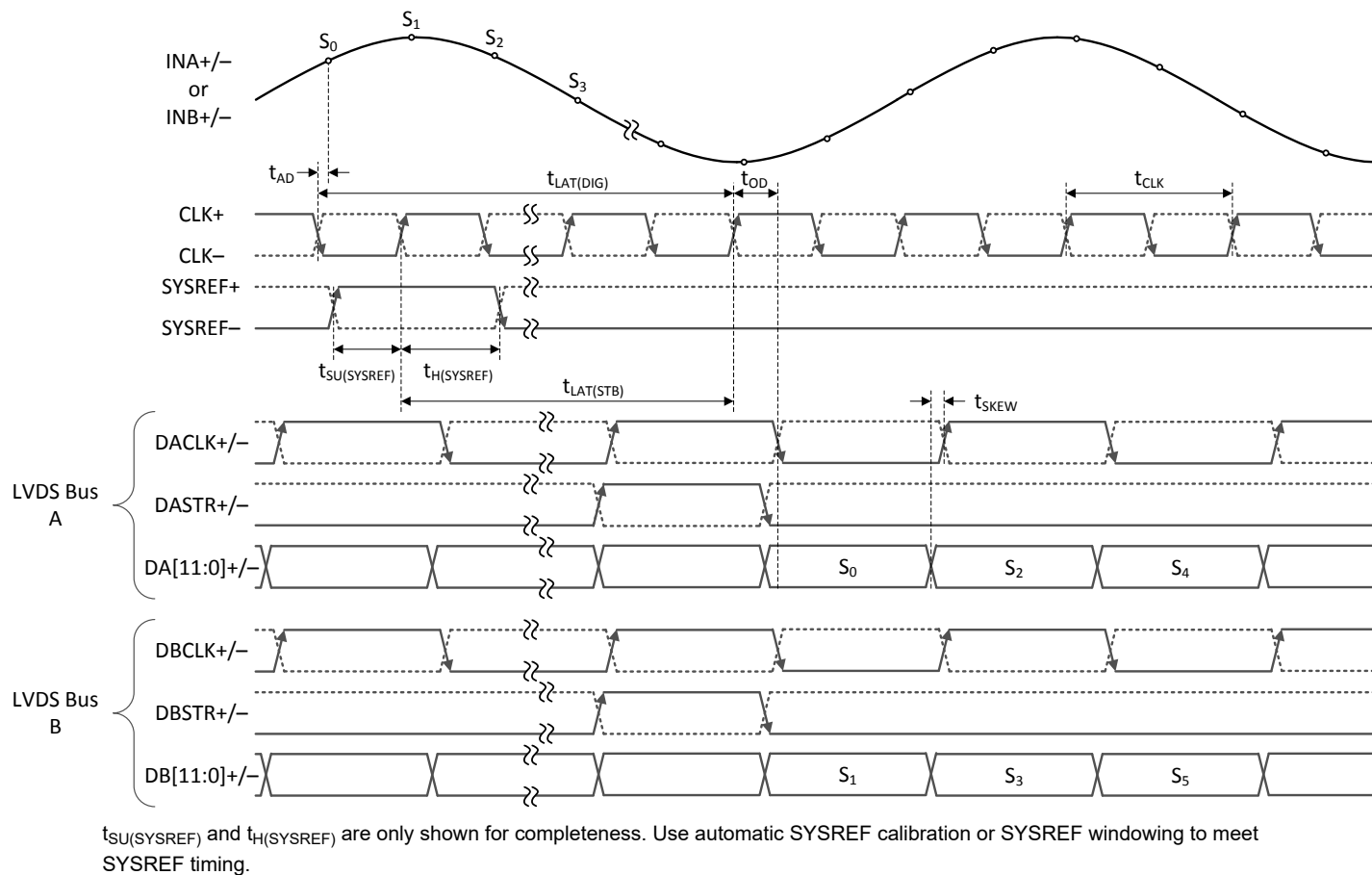
图 6-5. Single-Channel, 2-Bus, Aligned-Mode Timing (LDEMUX = 0, DES_EN = 1, LALIGNED = 1)
