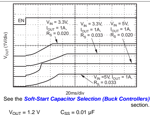
Figure 25. Buck Start-Up vs V_{IN} and R_{SENSE}
