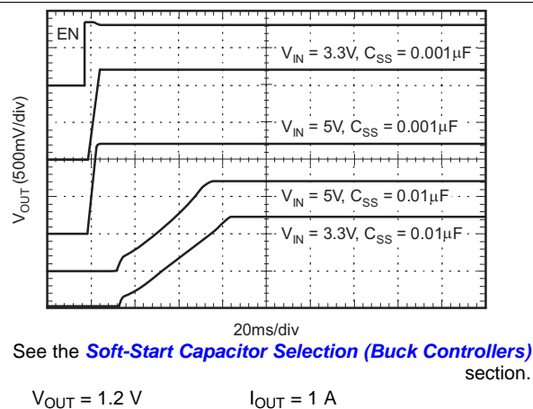
Figure 23. Buck Start-Up vs V_{IN} and C_{SS}
