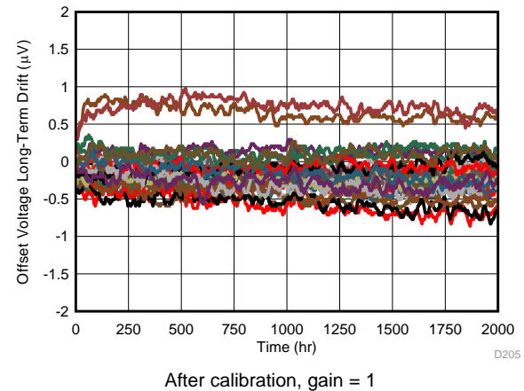
图 14. Offset Voltage Long-Term Drift
