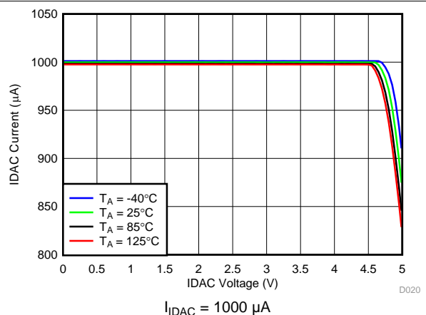
图 44. IDAC Current vs IDAC Voltage
