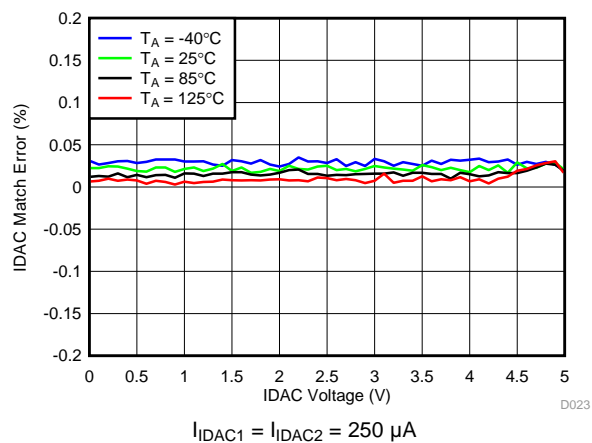
图 46. IDAC Current Match vs IDAC Voltage
