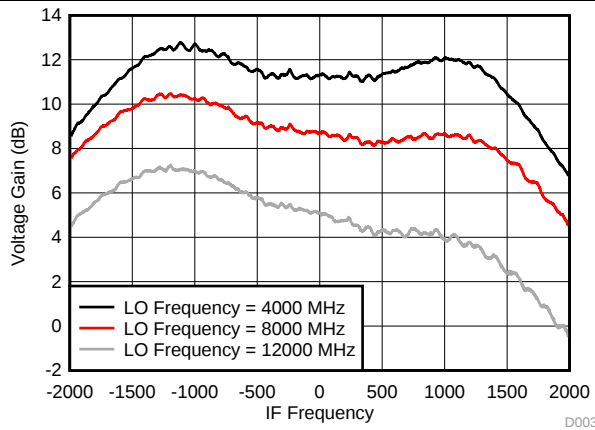
图 3. Voltage Gain Across LO Frequency for Internal LO Mode
