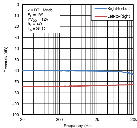
图 28. Crosstalk vs Frequency
