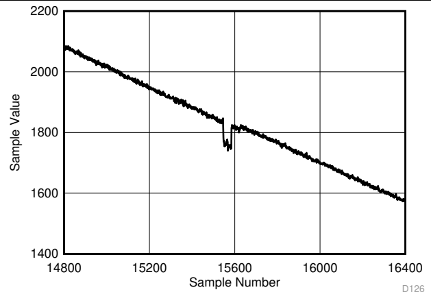
Figure 61. Background Calibration Core Transition (AC Signal Zoomed)
