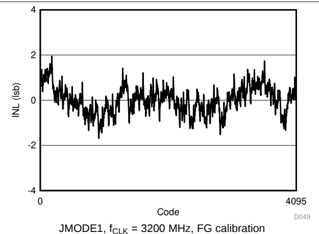
Figure 31. INL vs Code
