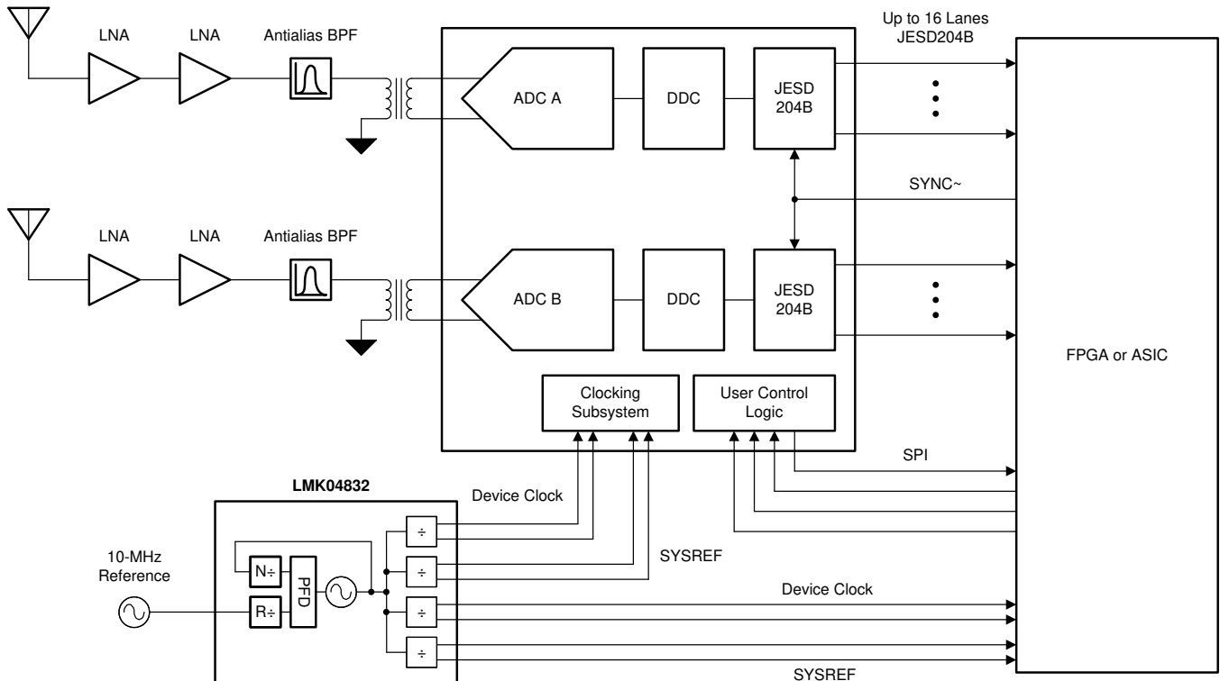
图 180. Typical Configuration for Wideband RF Sampling
