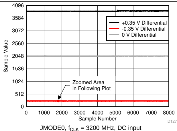
Figure 62. Background Calibration Core Transition (DC Signal)
