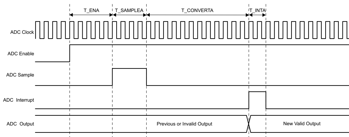
图 8-2. ADC Enable and Conversion Timing
