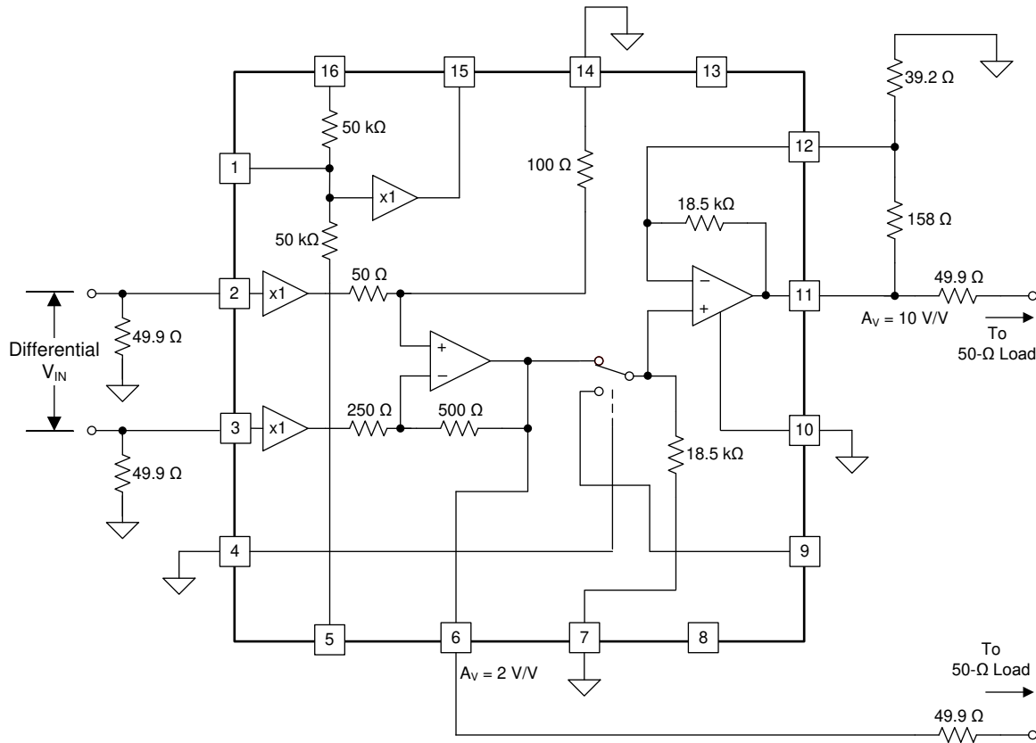
A simple modification to the circuit in 图 8-18 is to disable the OPS. The D2S output at VO1 can then be used either directly or through a filter to an even higher power driver, such as the \pm 15 V TSH3091 .
