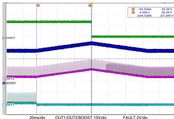
图 8-5. Open LED Fault
