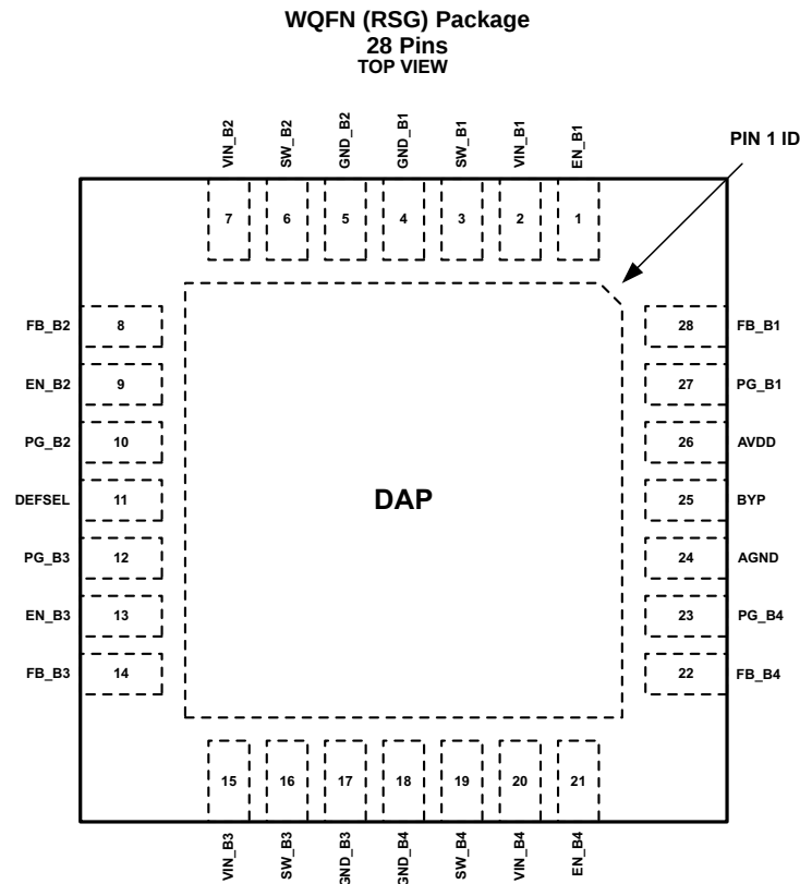
Pin Functions
