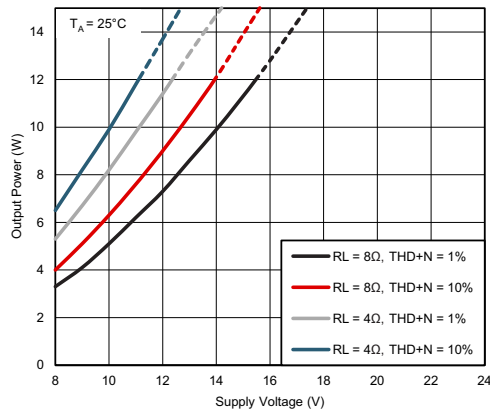
Figure 3. Output Power vs PVDD in BTL Mode
