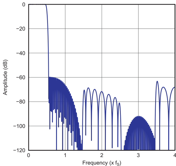
Figure 16. Normal ×8 Interpolation-Filter Frequency Response
