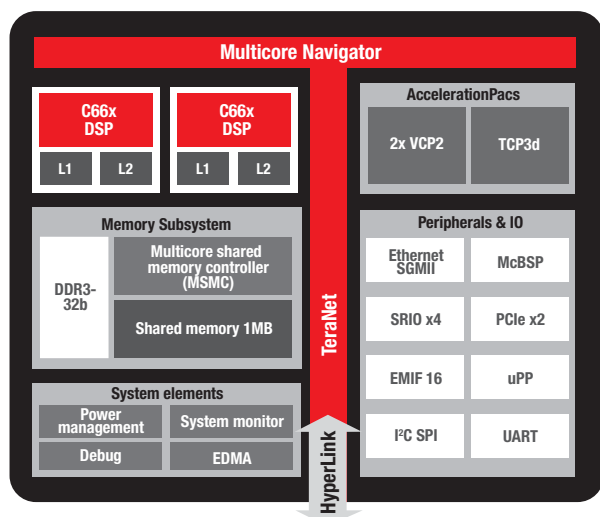
▲ Figure 1. TMS320C6657/55 block diagram
