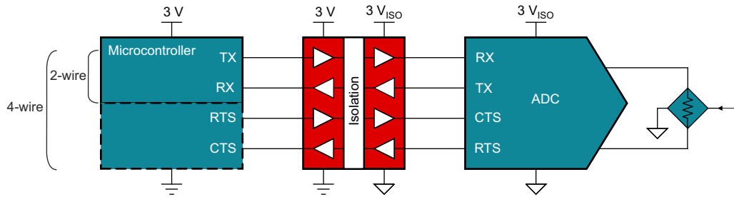
Example UART Isolation Block Diagram
