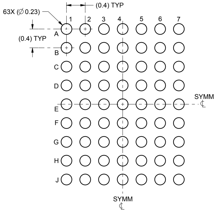
LAND PATTERN EXAMPLE SCALE:20X
