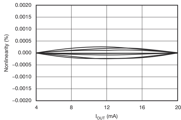
图 5-13. Typical Nonlinearity
