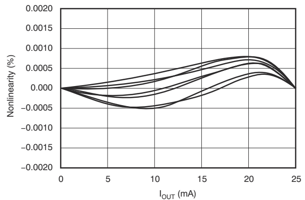
图 5-14. Typical Nonlinearity
