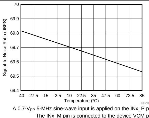
图 23. SNR vs Temperature For Single-Ended Input
