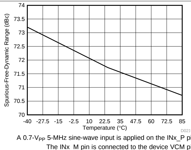
图 24. SFDR vs Temperature for Single-ended Input
