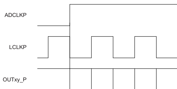
c) PHASE_DDR[1:0] = 01
