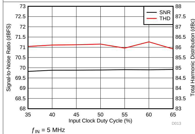
图 16. Performance vs Input Clock Duty Cycle
