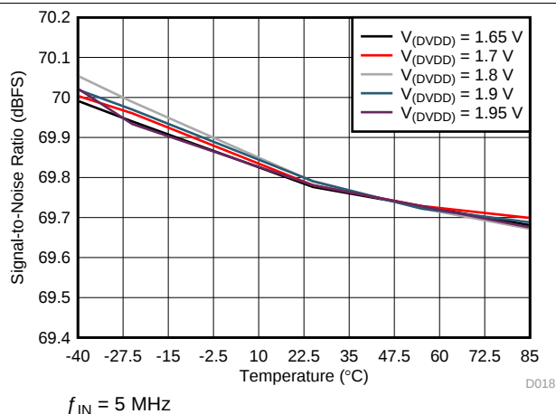
图 21. SNR vs DVDD and Temperature
