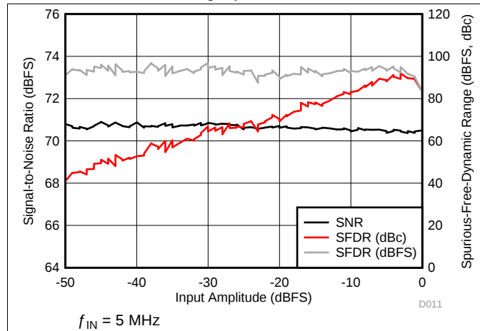
图 14. Performance vs Input Signal Amplitude
