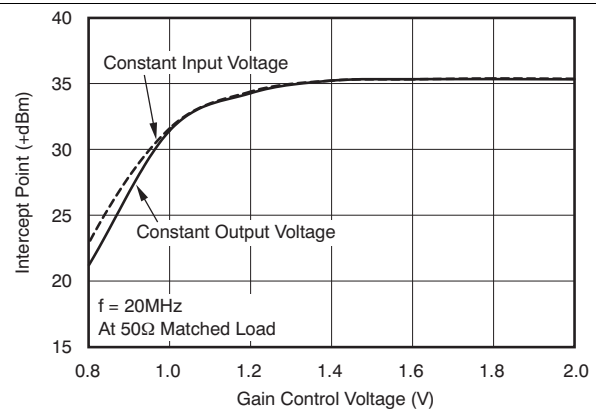
Figure 43. Two-Tone, Third-Order Intermodulation Intercept vs Gain Control Voltage
