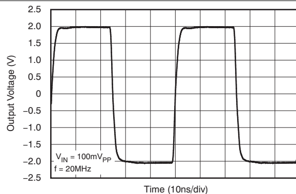
Figure 56. Large-Signal Pulse Response
