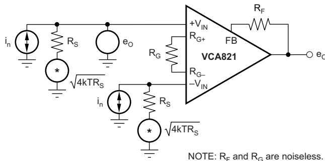
Figure 88. Simple Noise Model
