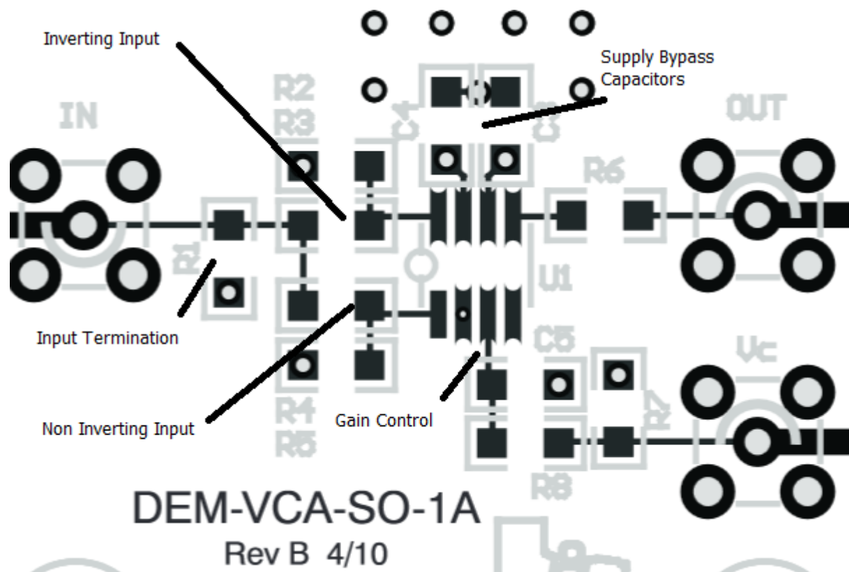
Figure 49. Layout Example
