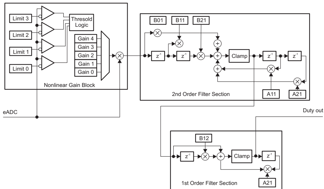
Figure 18. Digital Compensator
