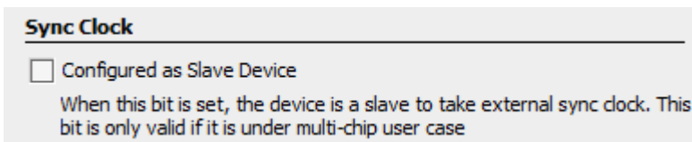
Figure 30. SYNC_CLK Pin Configuration (Global Configuration ► Misc Config)
