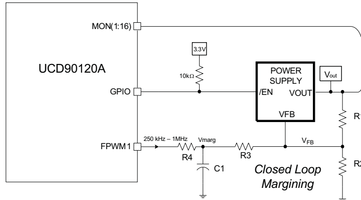
图 24. Closed-Loop Margining
