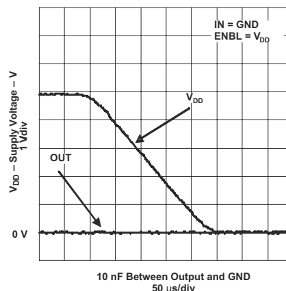
图 7-24. Output Behavior vs VDD (Noninverting)
