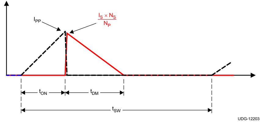
图 7-6. Transformer-Current Relationship
