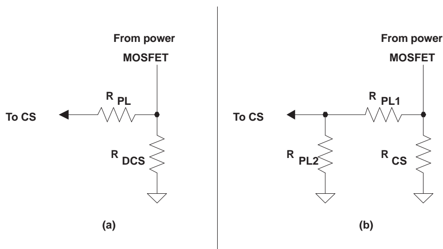
Figure 14. Modifications to Fit a Standard Current Sense Resistor Value
