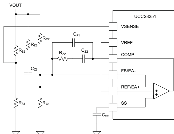
Figure 32. Error Amplifier EAMP Connections for Secondary-Side Control
