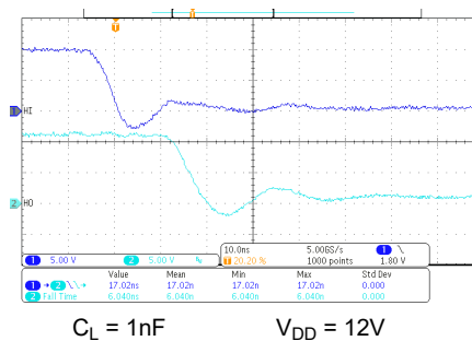
图 7-5. HO Fall Time and HI to HO Turn-off Propagation Delay
