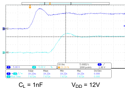
图 7-4. HO Rise Time and HI to HO Turn-on Propagation Delay
