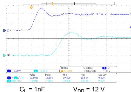
图 7-2. LO Rise Time and LI to LO Turn-on Propagation Delay
