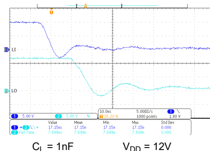
图 7-3. LO Fall Time and LI to LO Turn-off Propagation Delay
