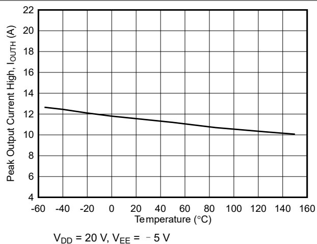
图 5-4. Output High Drive Current vs Temperature
