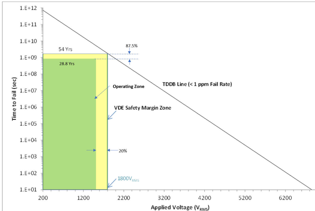
图 5-3. Reinforced Isolation Capacitor Lifetime Projection
