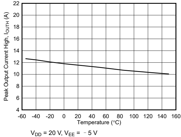
图 6-4. Output High Drive Current vs Temperature
