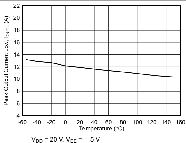
图 5-5. Output Low Driver Current vs Temperature
