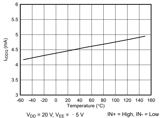
图 6-9. I_{VDDQ} Supply Current vs Temperature
