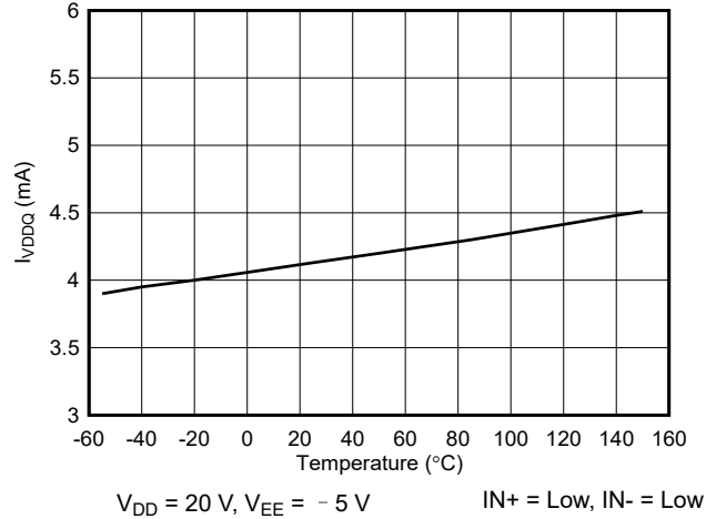
图 6-10. I_{VDDQ} Supply Current vs Temperature
