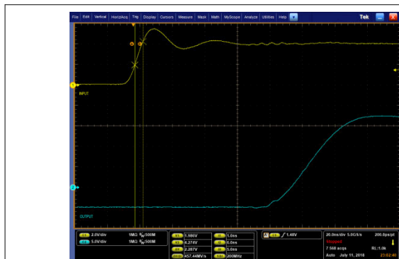
图 9-12. PWM Input (yellow) and Driver Output (blue) Rising Edge
