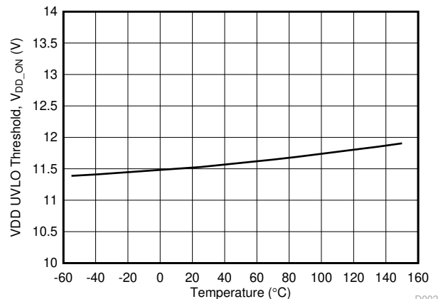
图 5-13. VDD UVLO vs Temperature
