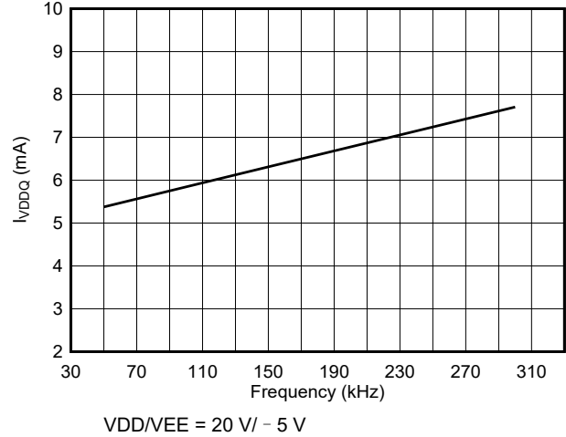
图 6-11. I_{VDDQ} Supply Current vs Input Frequency
