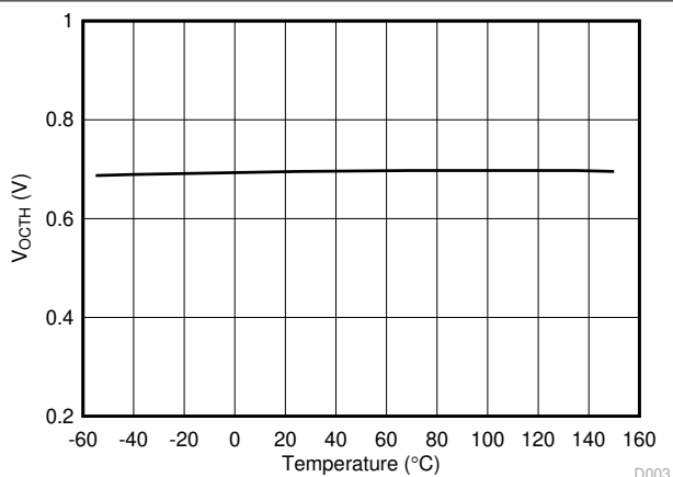
图 5-24. V_{OCTH} OC Detection Threshold vs Temperature
