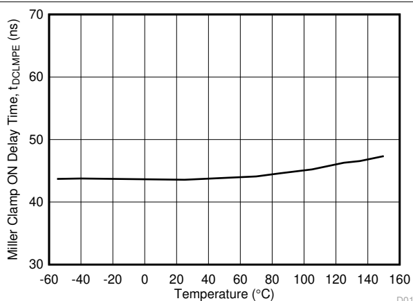
图 5-23. t_{DCLMPE} Miller Clamp ON Delay Time vs Temperature
