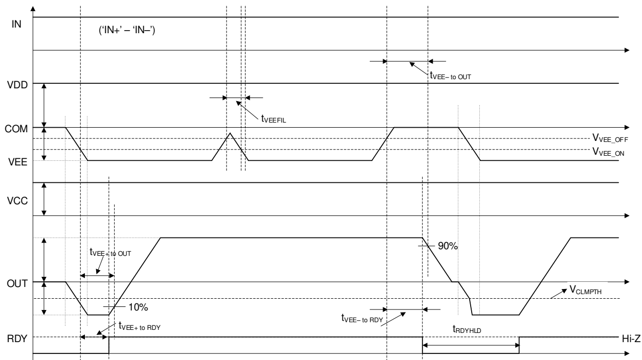
图 7-10. VEE UVLO Protection Timing Diagram
