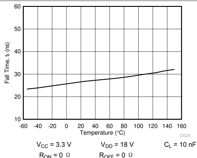
图 5-17. t_f Fall Time vs Temperature
