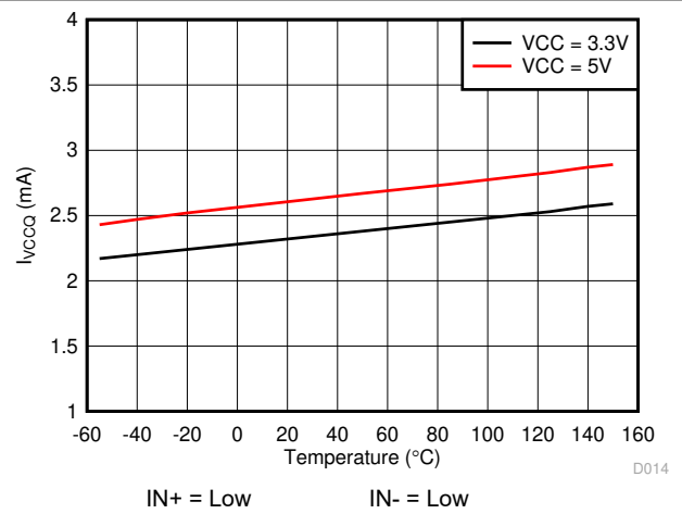
图 6-7. I_{VCCQ} Supply Current vs Temperature
