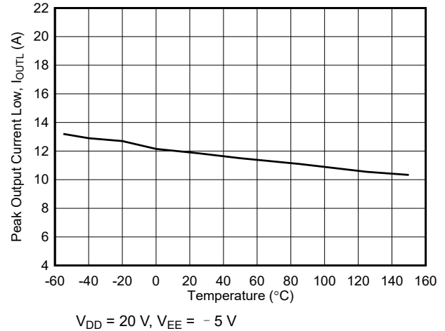
图 6-5. Output Low Driver Current vs Temperature
