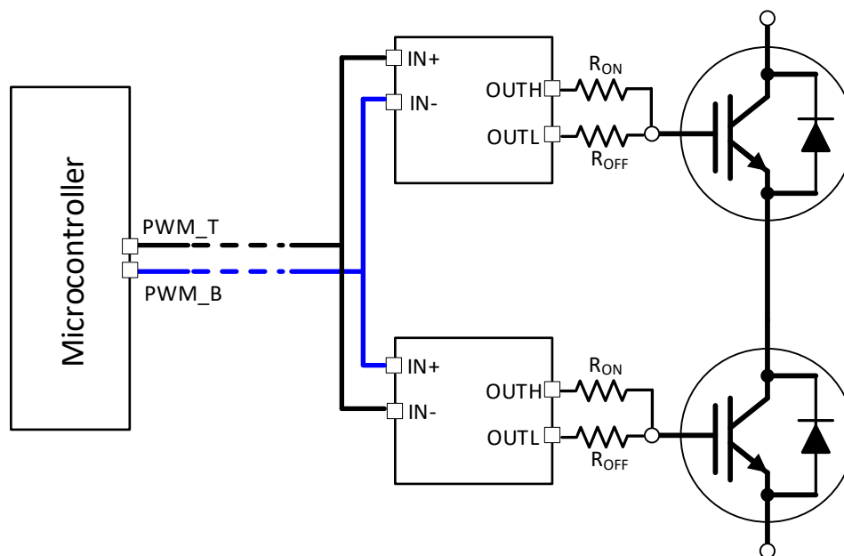
图 45. PWM Interlock for a Half Bridge
