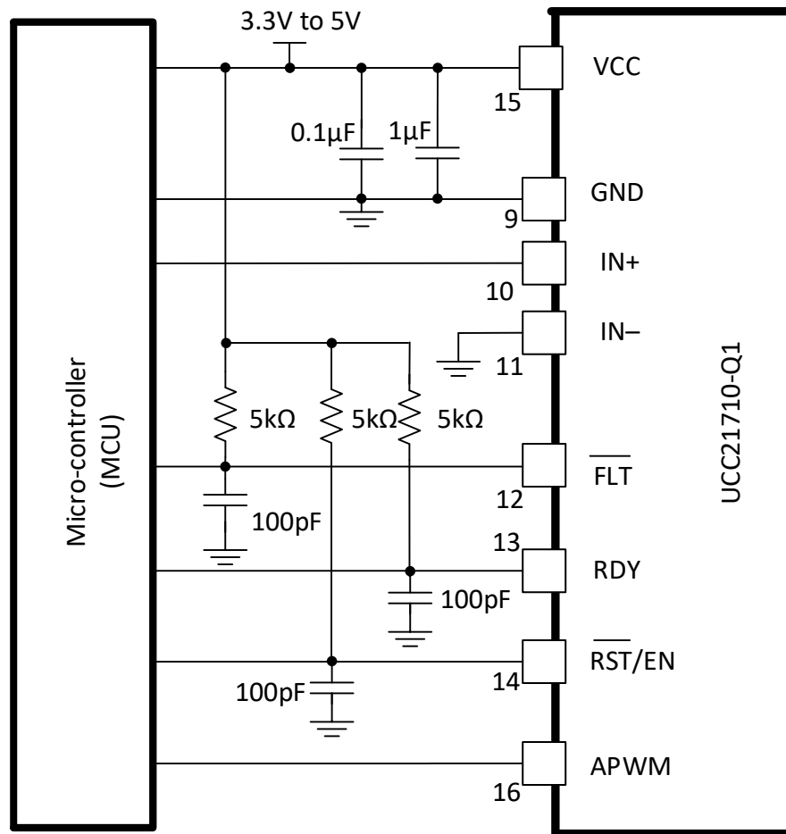
图 9-3. \overline{\text{FLT}} , RDY and \overline{\text{RST/EN}} Pins Circuitry
