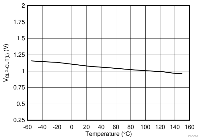
图 6-20. V_{CLP-OUT(L)} Short Circuit Clamping Voltage vs. Temperature
