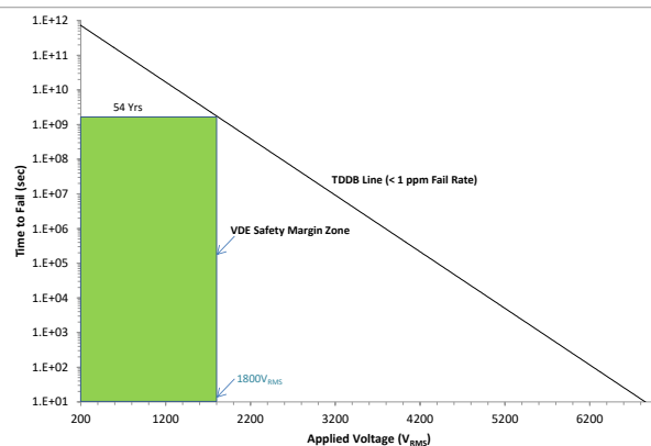
图 6-3. Reinforced Isolation Capacitor Life Time Projection
