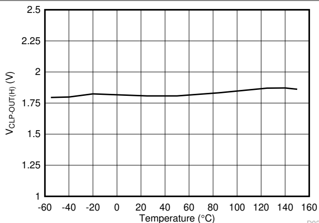
图 6-19. V_{CLP-OUT(H)} Short Circuit Clamping Voltage vs. Temperature
