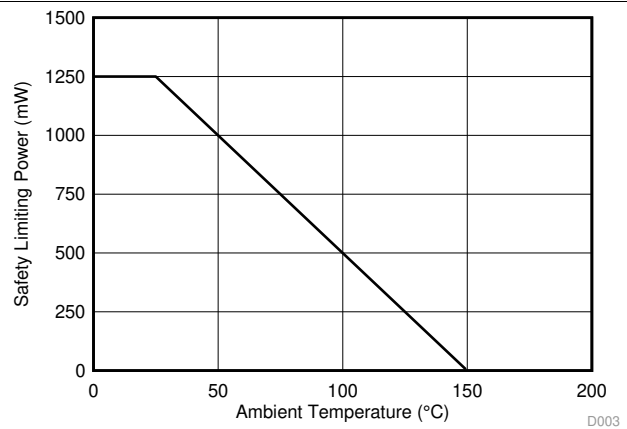
图 3. Thermal Derating Curve for Safety-Related Limiting Power
