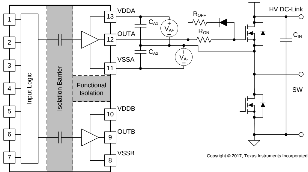
图 37. Negative Bias with Two Iso-Bias Power Supplies
