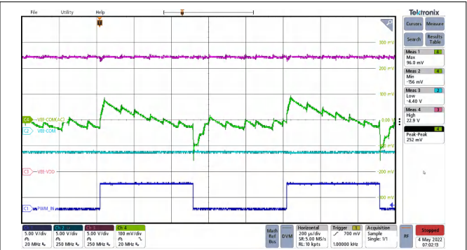
图 8-5. Ripple voltage: VEE-COM Switching 100-nF Load at 1 kHz.
