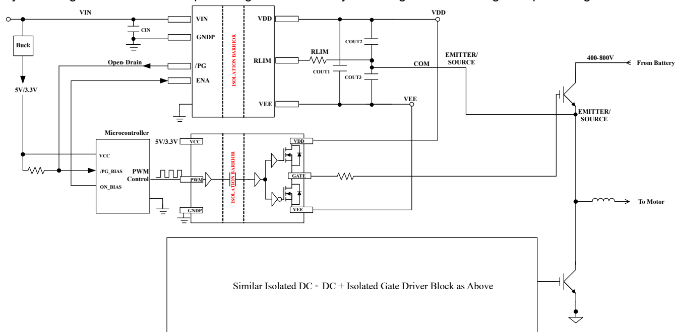
图 8-11. Dual Output System Configuration
