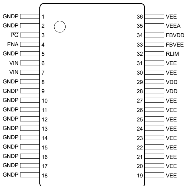
图 5-1. DWN Package, 36-Pin SSOP (Top View)
