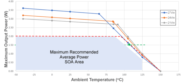
图 6-3. SOA Derating Curves: V_{DD-VEE} = 20\text{ V} , V_{COM-VEE} = 5\text{ V} , No Load
