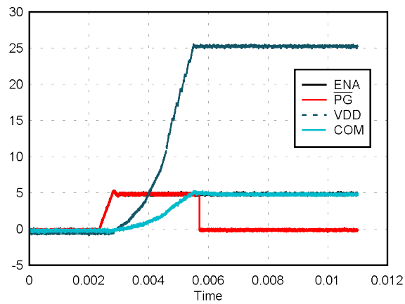
图 6-5. Start-up: V_{IN} = 24\text{ V} , V_{DD-VEE} = 25\text{ V} , V_{COM-VEE} = 5\text{ V} , No Load
