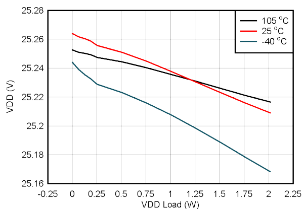
图 6-10. V_{DD-VEE} Load Regulation: V_{IN} = 24\text{ V} , V_{DD-VEE} = 25\text{ V} , V_{COM-VEE} = 5\text{ V}
