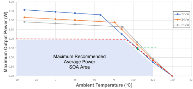
图 6-2. SOA Derating Curves: V_{DD-VEE} = 18\text{ V} , V_{COM-VEE} = 5\text{ V} , No Load.
