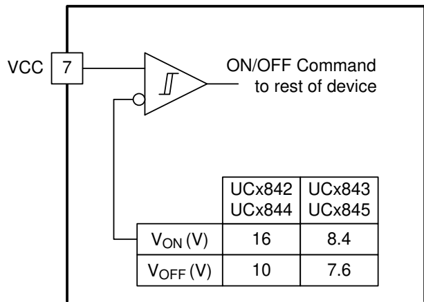
Copyright © 2016, Texas Instruments Incorporated 图 7-5. UVLO 阈值
