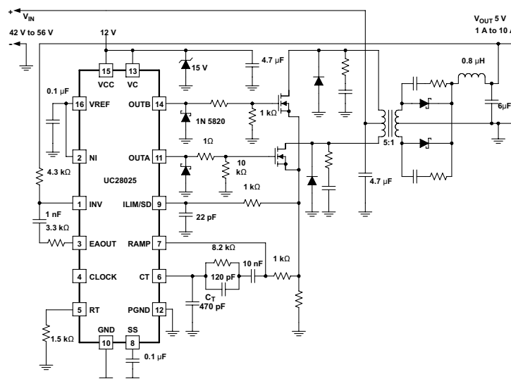
Typical Application Schematic
