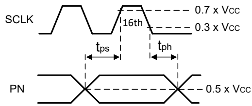
READ MODE ( \overline{R}/\overline{W} = 1 )
