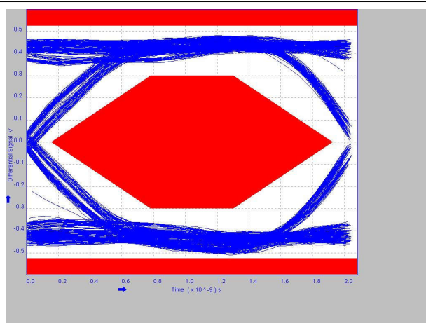
图 6-1. 2 Meter Pre-Channel With TUSB211A EQ=1
