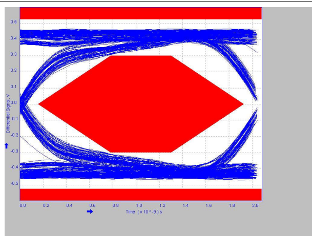
图 8-3. 2 Meter Pre-Channel Without TUSB211A
