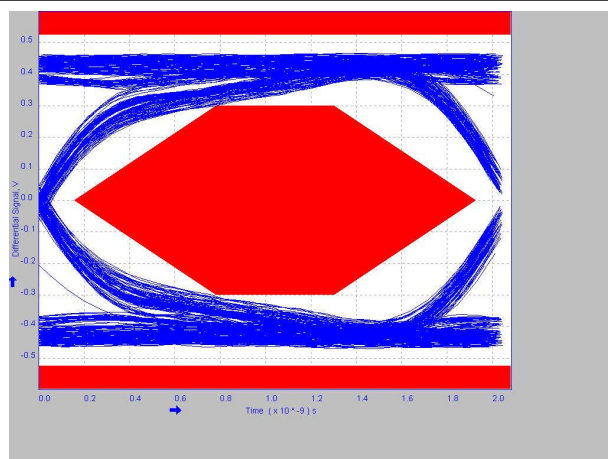
图 8-11. 2 Meter Post-Channel Without TUSB211A
