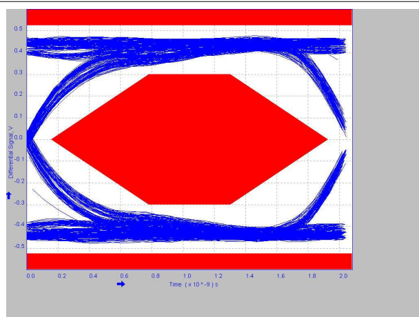
图 8-9. 1 Meter Post-Channel Without TUSB211A
