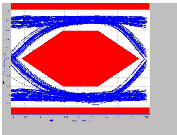
图 6-4. 4 Meter Post-Channel With TUSB211A EQ=2
