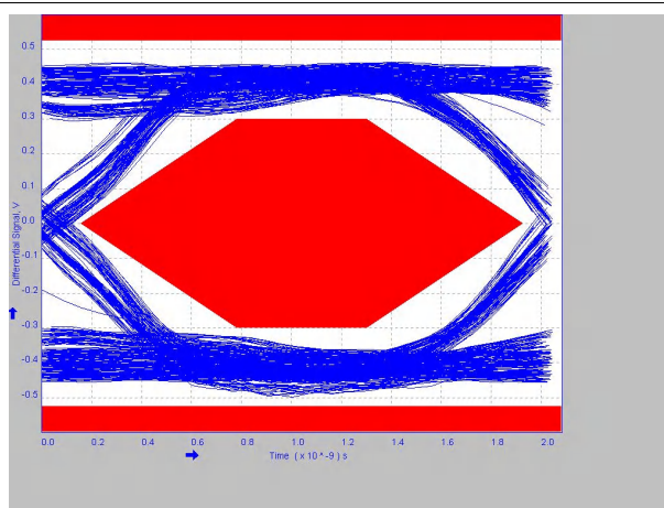
图 6-2. 5 Meter Pre-Channel With TUSB211A EQ=2
