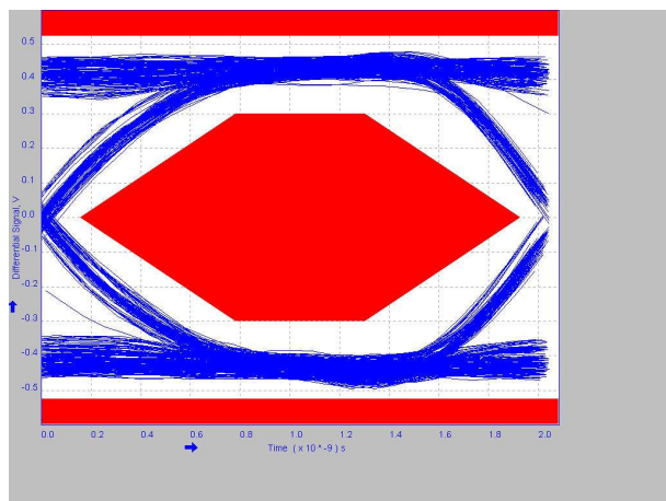
图 6-3. 2 Meter Post-Channel With TUSB211A EQ=1
