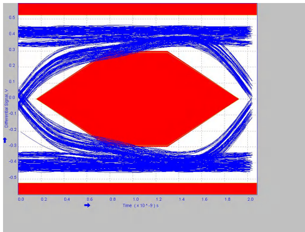
图 8-13. 4 Meter Post-Channel Without TUSB211A
