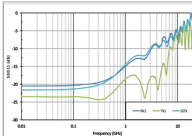
图 7. Input Return Loss Performance
