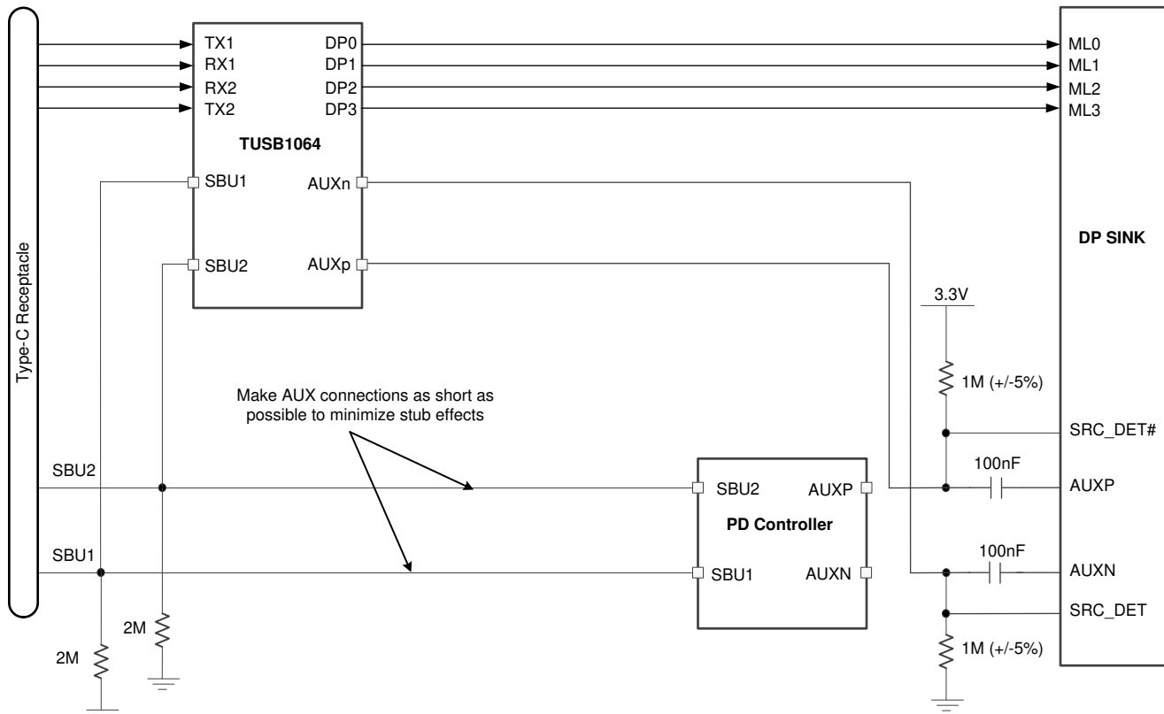
图 28. DisplayPort AUX Connections for UFP_D Pin Assignment E with Internal AUX Switching
