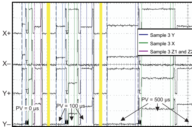
图 54. Panel Voltage Stabilization 0 \mu s, 100 \mu s, and 500 \mu s
