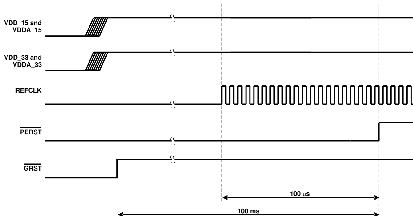
图 10-2. Power-Up Sequence
