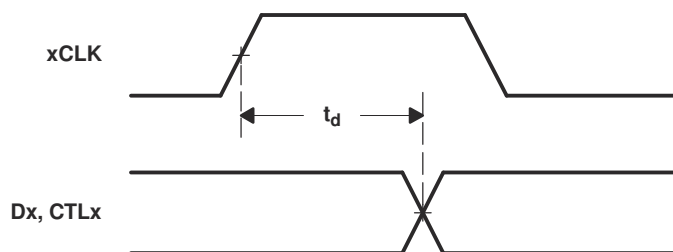
图 9-2. Dx and CTLx Output Delay Relative to xCLK Waveforms
