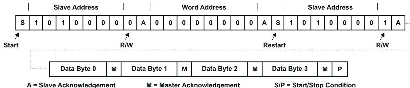
图 10-11. Serial-Bus Protocol Multibyte Read
