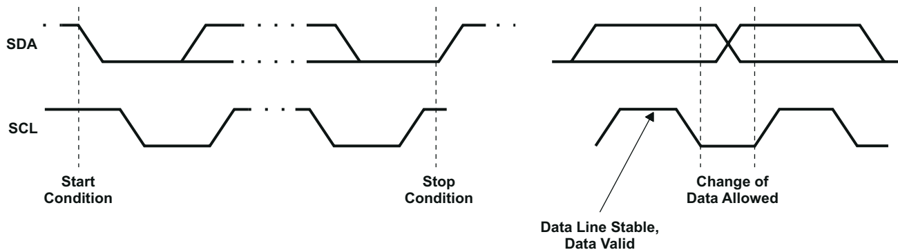
图 10-7. Serial-Bus Start/Stop Conditions and Bit Transfers
