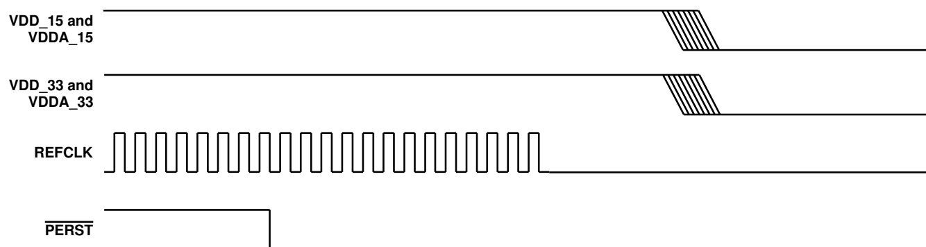
图 10-3. Power-Down Sequence
