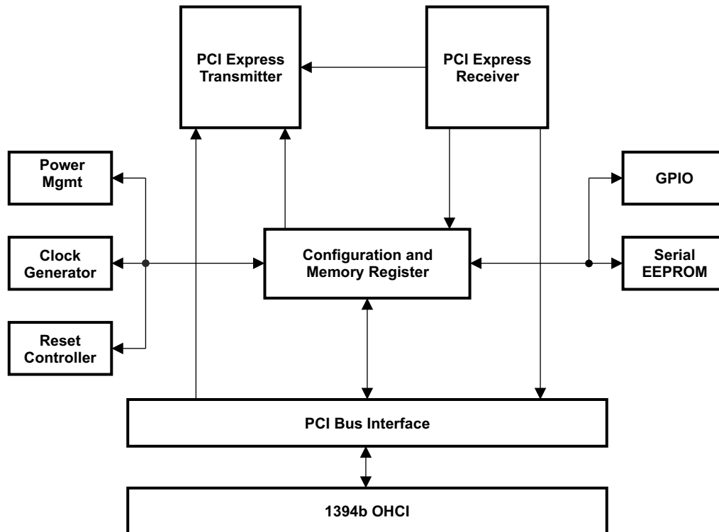
图 10-1. TSB82AF15-EP Block Diagram
