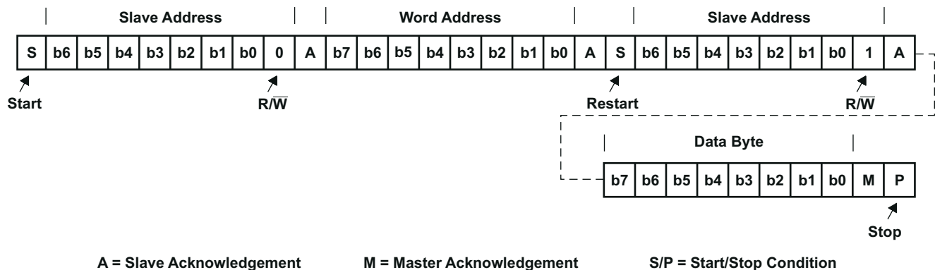
图 10-10. Serial-Bus Protocol Byte Read
