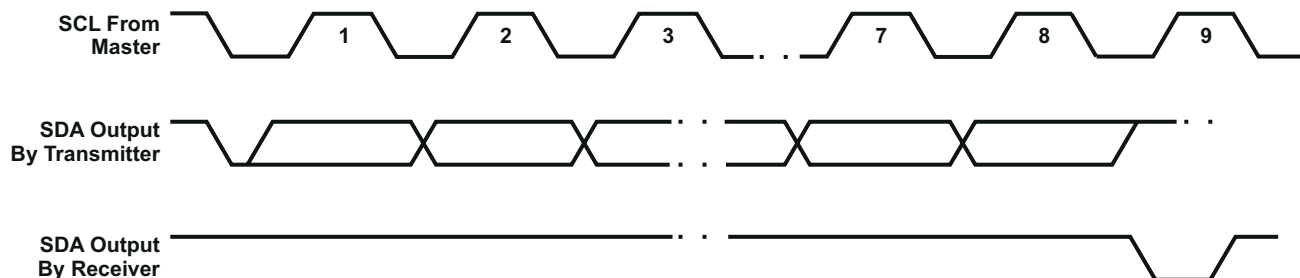
图 10-8. Serial-Bus Protocol Acknowledge
