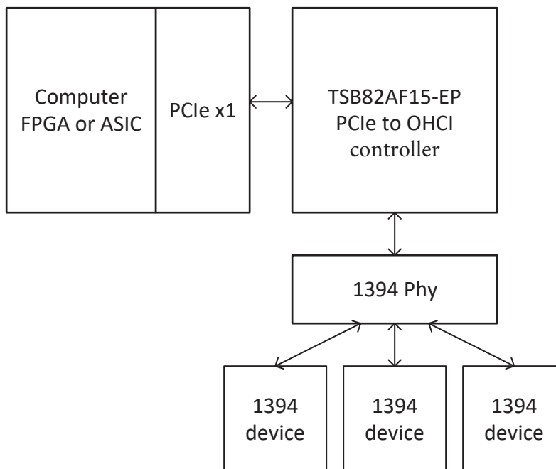
图 11-1. Typical application example
