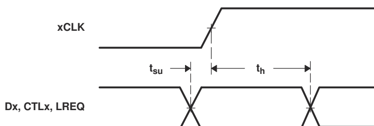
图 9-1. Dx, CTLx, LREQ Input Setup and Hold Time Waveforms
