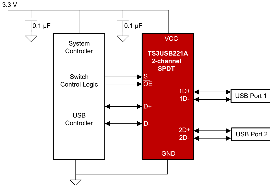
图 8-1. Application Schematic
