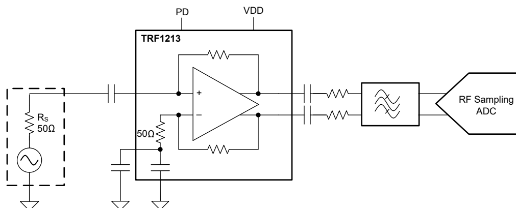
TRF1213 驱动射频采样 ADC
