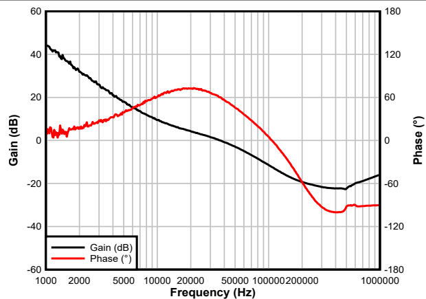
图 8-8. Total-Loop Bode Plot
