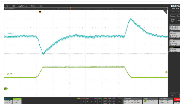
图 8-12. Load Transient Response
