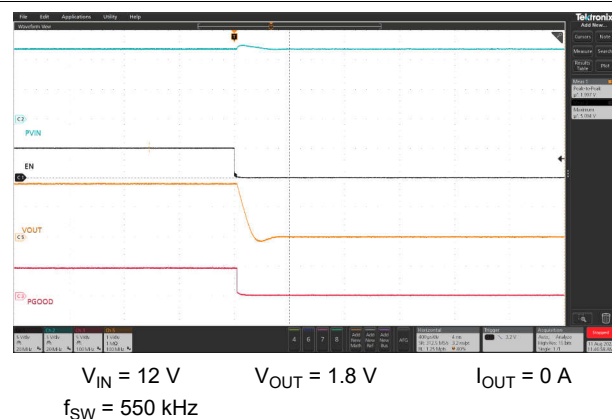
图 8-22. Shutdown from CNTL
