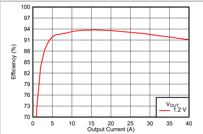
图 8-3. VOUTB Efficiency
