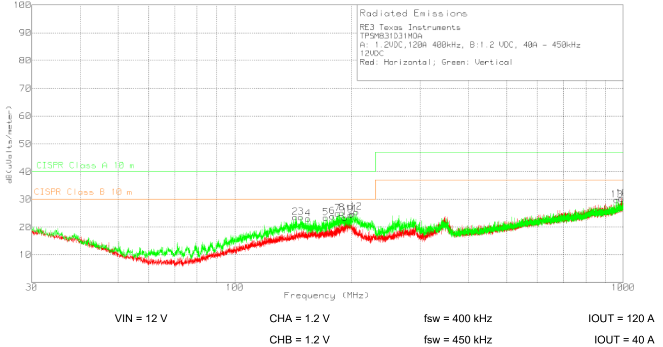
图 8-16. Radiated EMI
