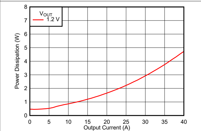
图 8-5. VOUTB Power Dissipation
