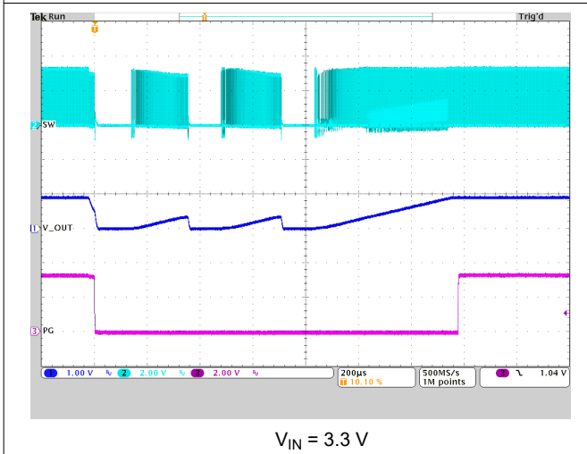
图 9-34. Current Limit (Hiccup)
