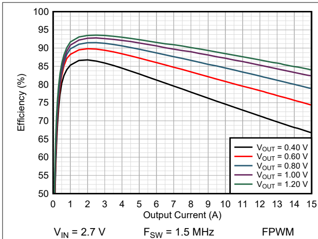
图 9-14. Efficiency TPSM8287A15BAH
