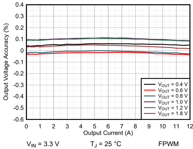
图 9-22. Load Regulation TPSM8287A12BAS
