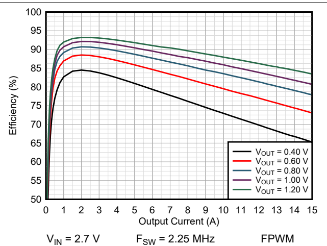
图 9-15. Efficiency TPSM8287A15BBH
