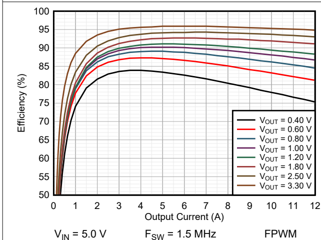
图 9-12. Efficiency TPSM8287A12BAS
