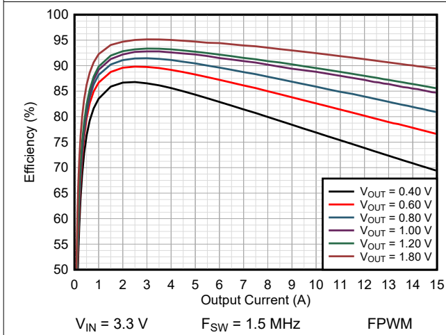
图 9-16. Efficiency TPSM8287A15BAH
