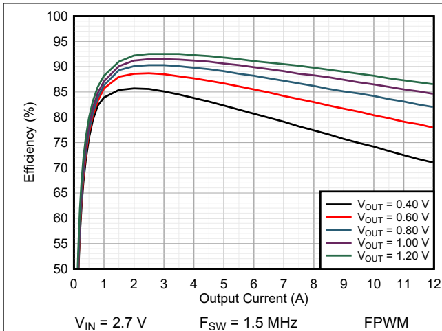
图 9-8. Efficiency TPSM8287A12BAS
