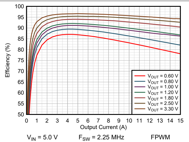
图 9-19. Efficiency TPSM8287A15BBH
