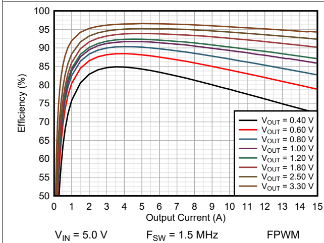
图 9-18. Efficiency TPSM8287A15BAH
