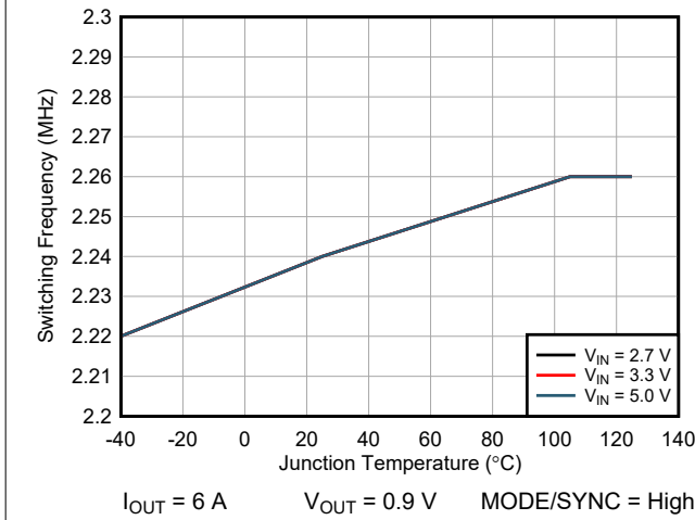
图 6-3. TPSM8287A12BBS Switching Frequency vs T J
