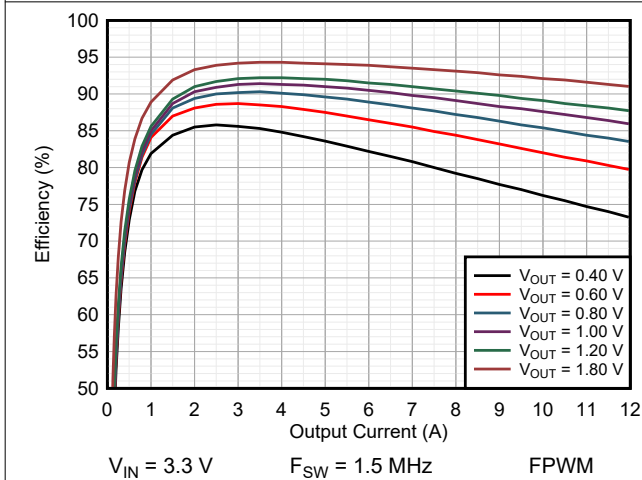
图 9-10. Efficiency TPSM8287A12BAS
