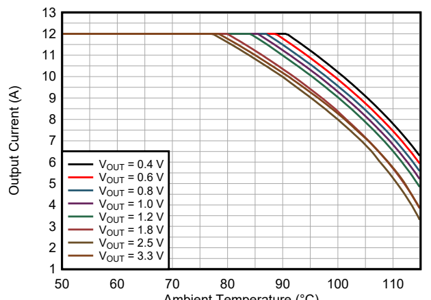
图 9-41. Safe Operating Area TPSM8287A10BAH V_{IN} = 5.0\text{ V}
