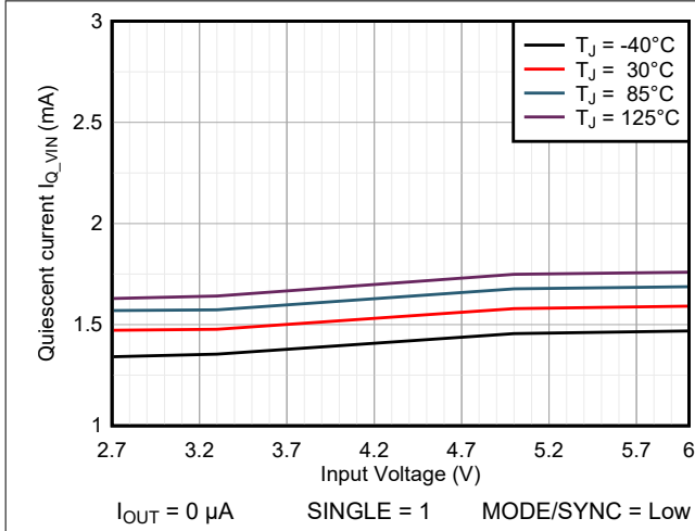
图 6-1. Operating Supply Current (Power-Save Mode)
