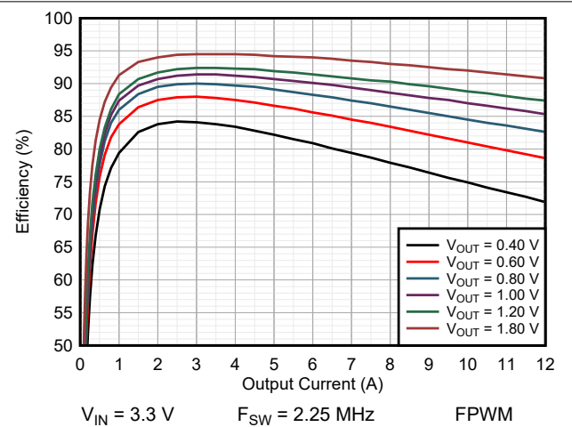
图 9-11. Efficiency TPSM8287A12BBS
