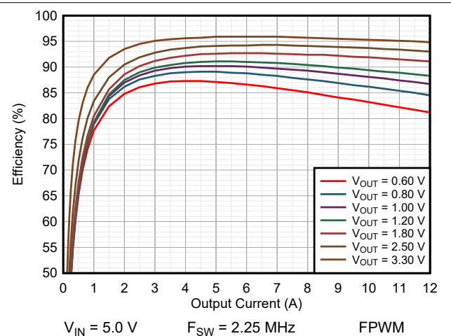
图 9-13. Efficiency TPSM8287A12BBS
