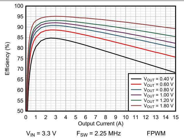
图 9-17. Efficiency TPSM8287A15BBH
