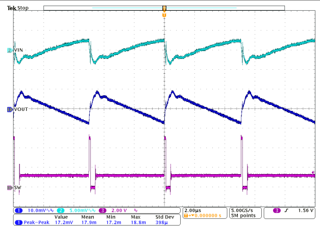
图 8-27. Switching Frequency V_{IN} = 3.3\text{ V}
