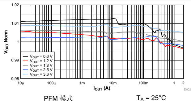
图 9-14. 负载调整率 ( V_{IN} = 5V )
